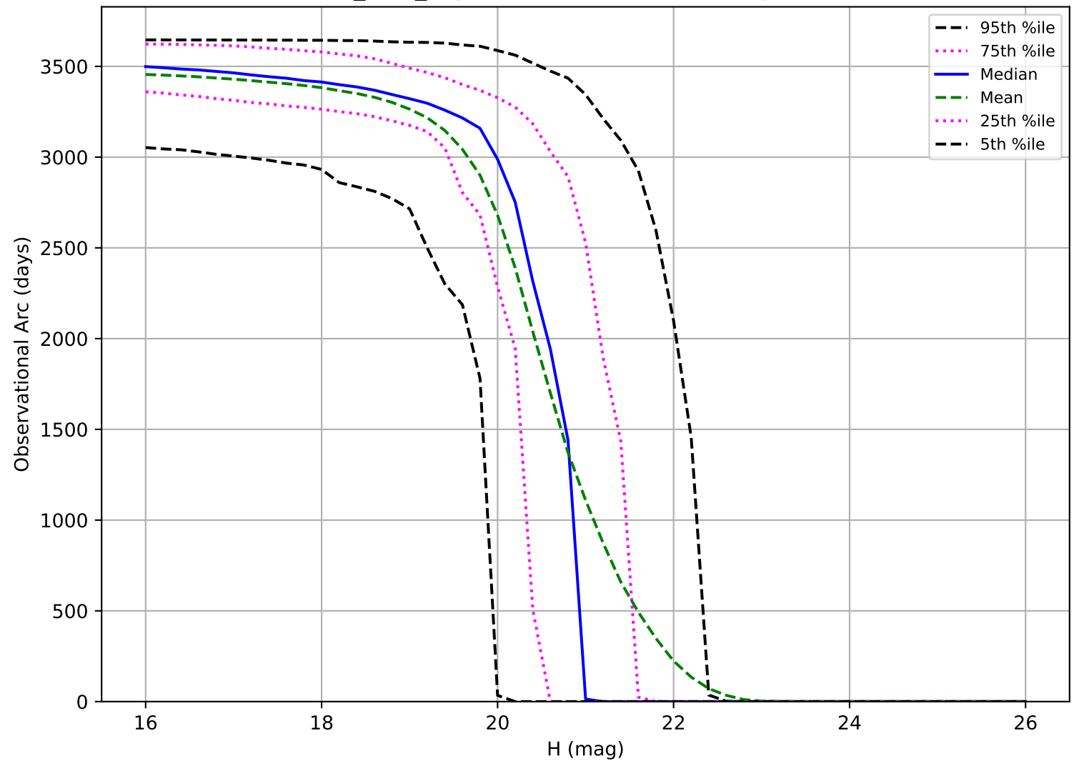
too_v3.5_10yrs: Observational Arc Length MBA
