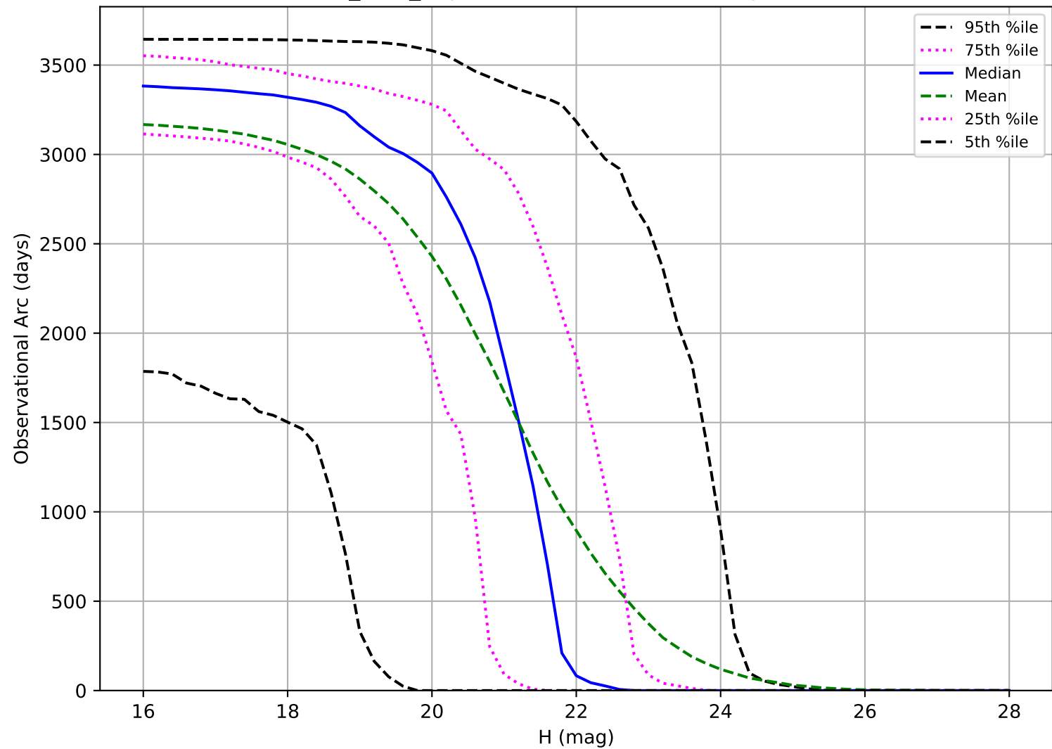
too_v3.5_10yrs: Observational Arc Length NEO
