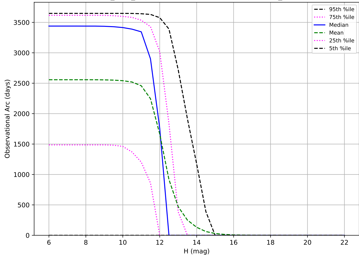
too_v3.5_10yrs: Observational Arc Length OCC_r20
