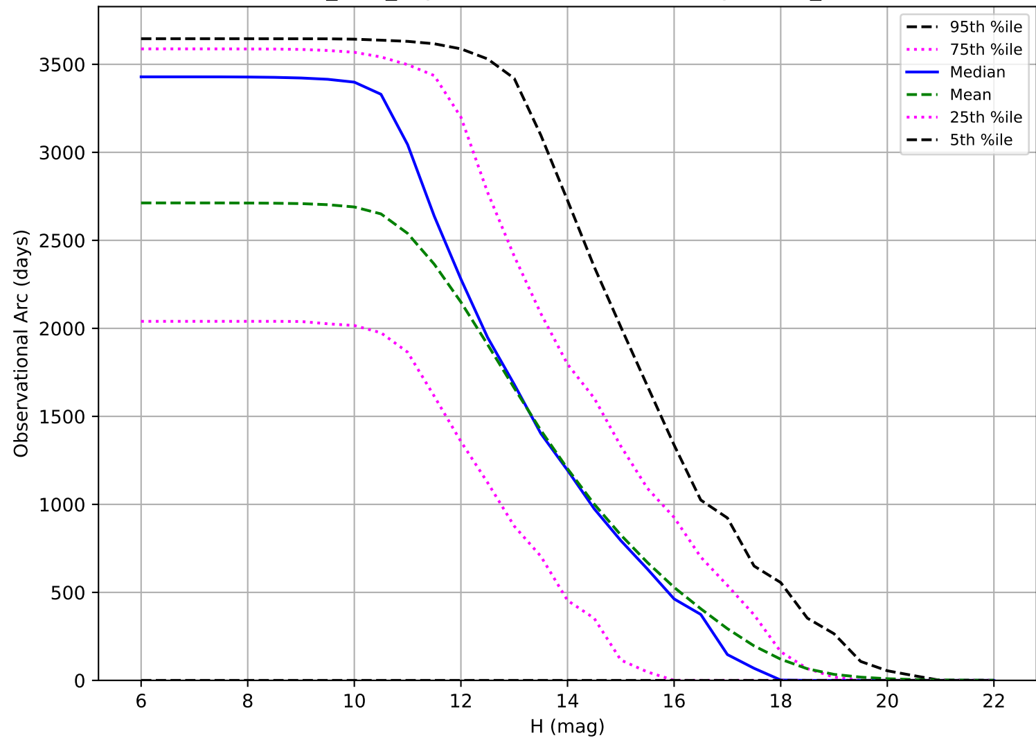
too_v3.5_10yrs: Observational Arc Length OCC_r5
