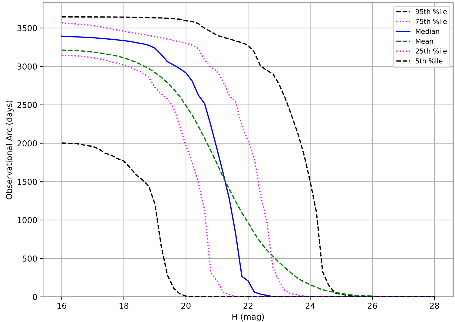
too_v3.5_10yrs: Observational Arc Length PHA
