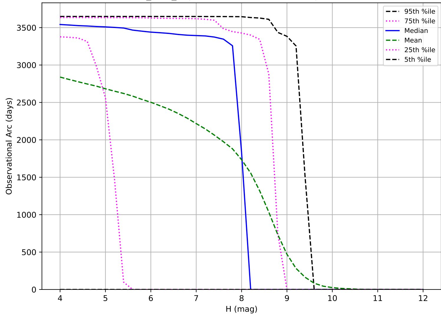
too_v3.5_10yrs: Observational Arc Length TNO
