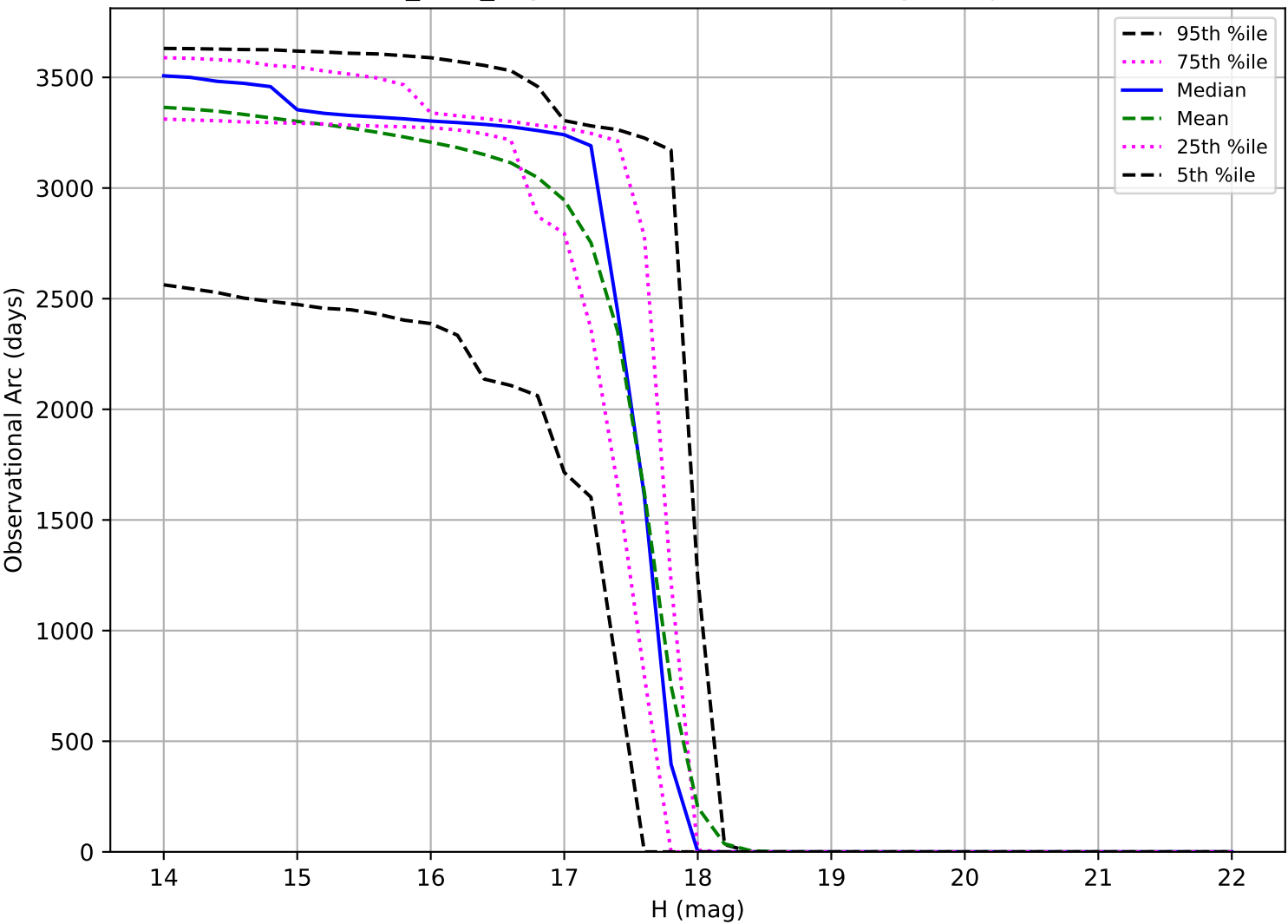
too_v3.5_10yrs: Observational Arc Length Trojan
