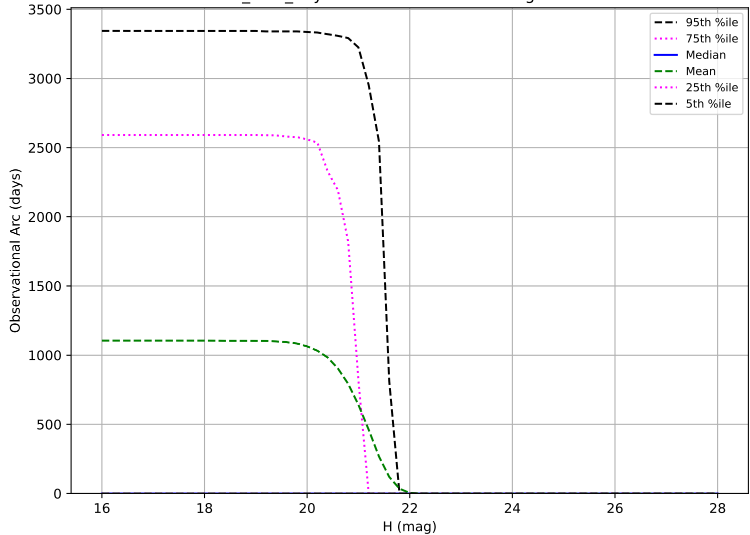
too_v3.5_10yrs: Observational Arc Length Vatira
