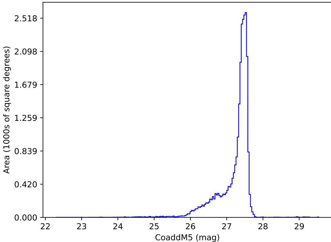
weather_cloudso0v3.5_10yrs : CoaddM5
