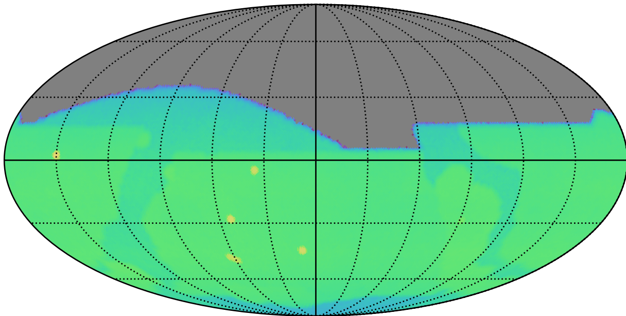
weather_cloudso0v3.5_10yrs : CoaddM5
