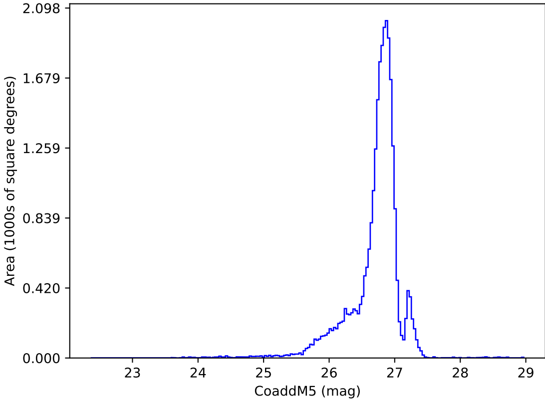
weather_cloudso0v3.5_10yrs g: CoaddM5
