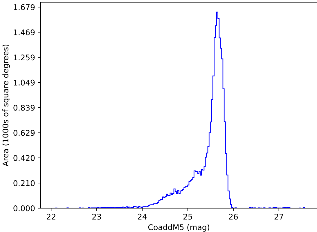
weather_cloudso0v3.5_10yrs u: CoaddM5
