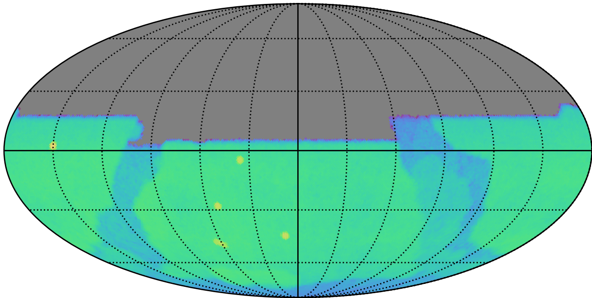
weather_cloudso0v3.5_10yrs u: CoaddM5
