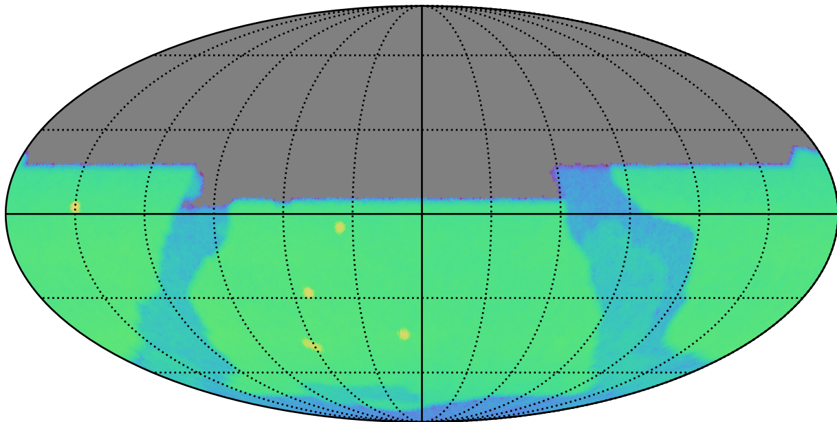
weather_cloudso0v3.5_10yrs y: CoaddM5
