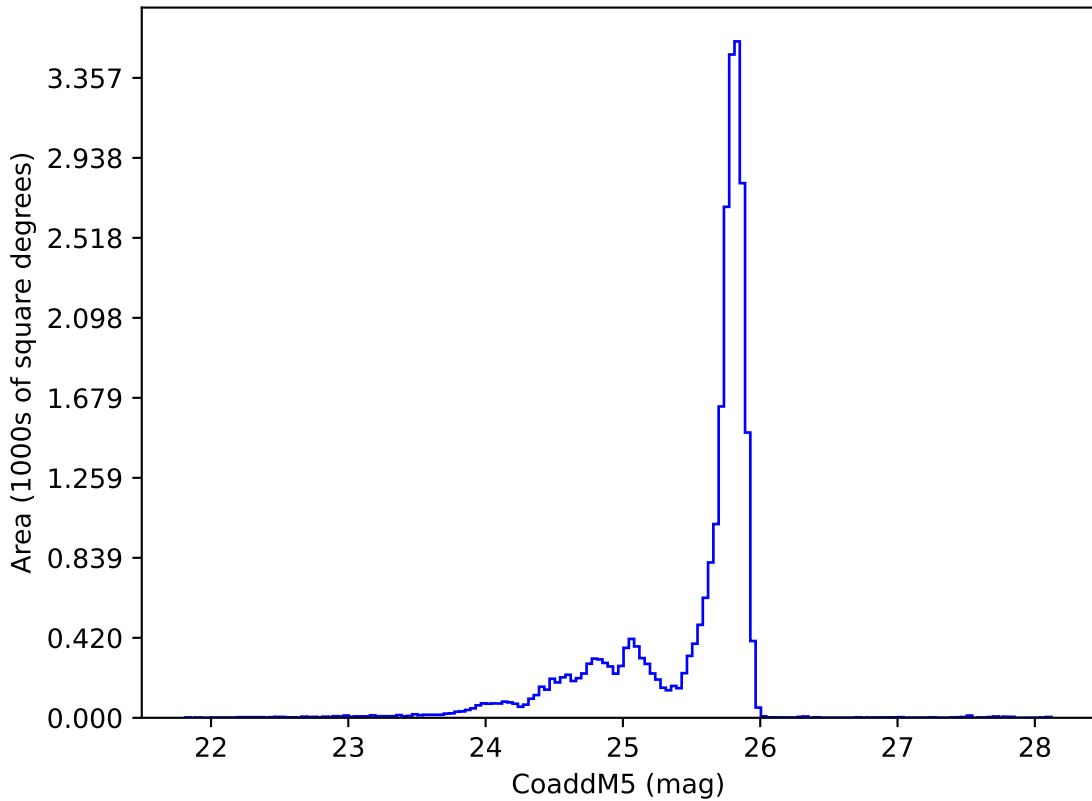
weather_cloudso0v3.5_10yrs z: CoaddM5
