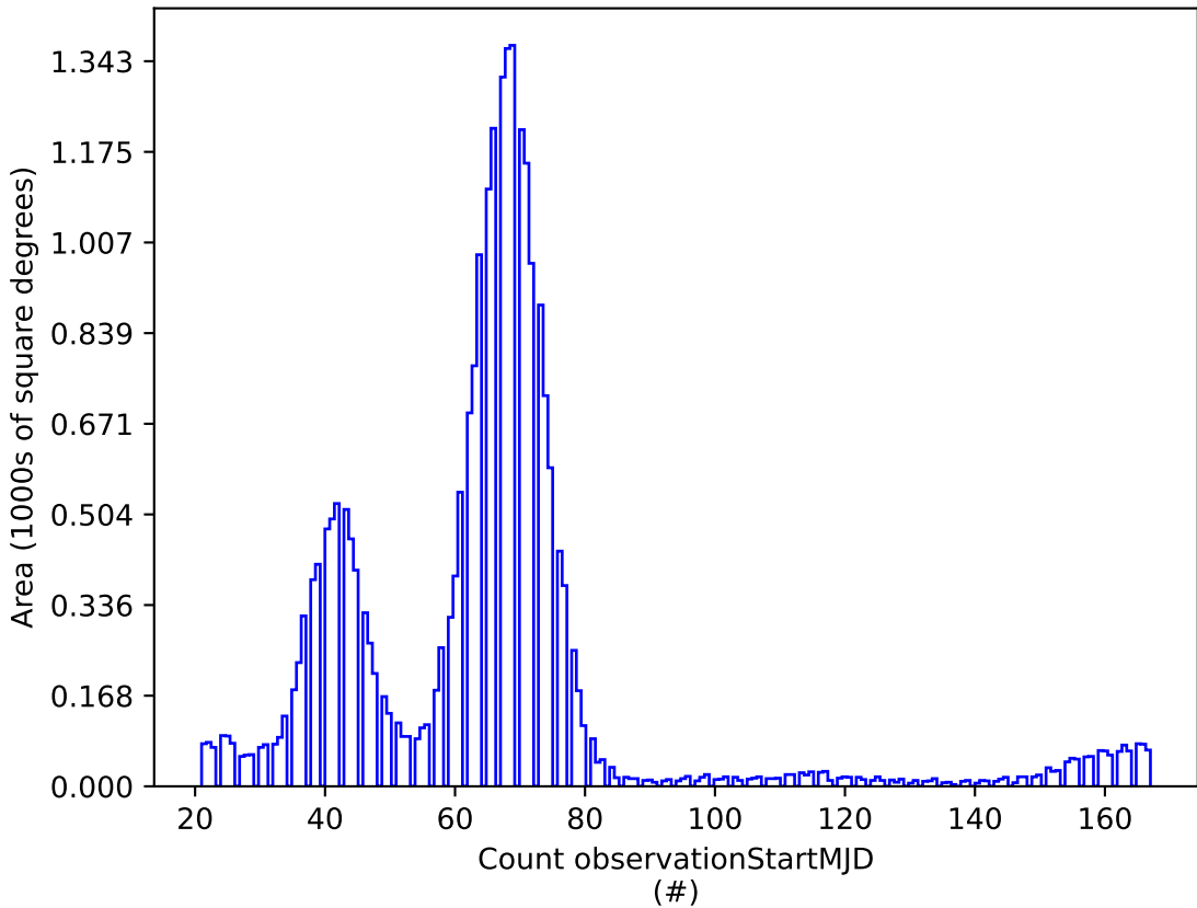
weather_cloudso0v3.5_10yrs g: Count observationStartMJD
