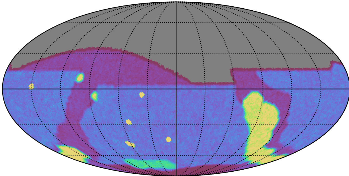
weather_cloudso0v3.5_10yrs g: Count observationStartMJD
