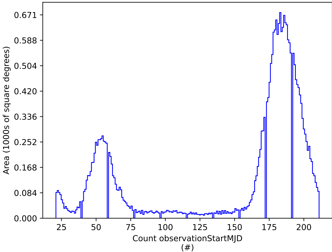
weather_cloudso0v3.5_10yrs i: Count observationStartMJD
