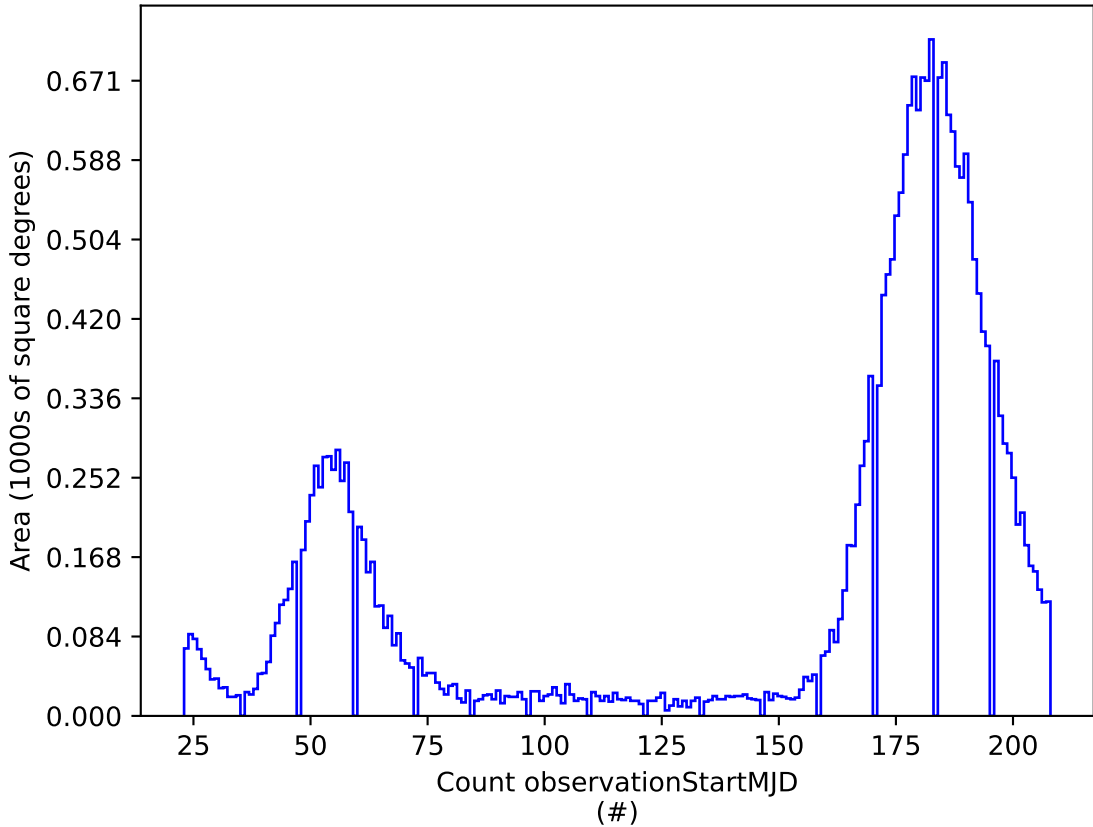
weather_cloudso0v3.5_10yrs r: Count observationStartMJD
