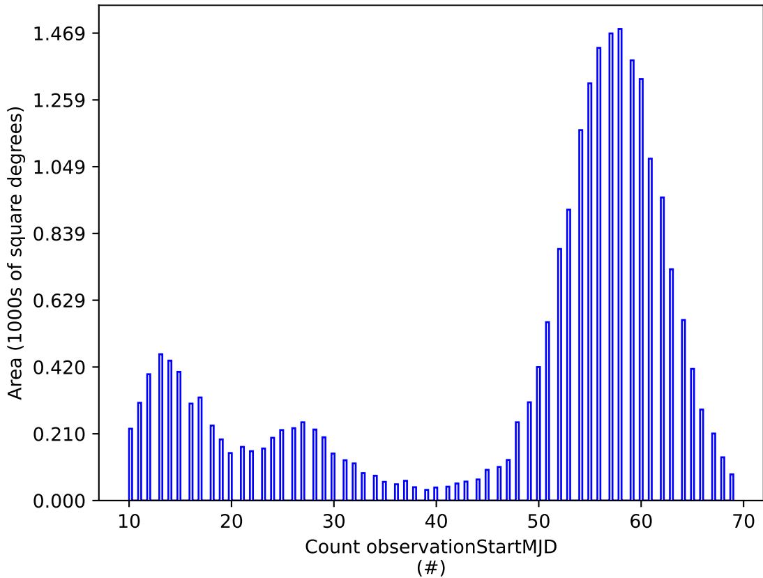
weather_cloudso0v3.5_10yrs u: Count observationStartMJD
