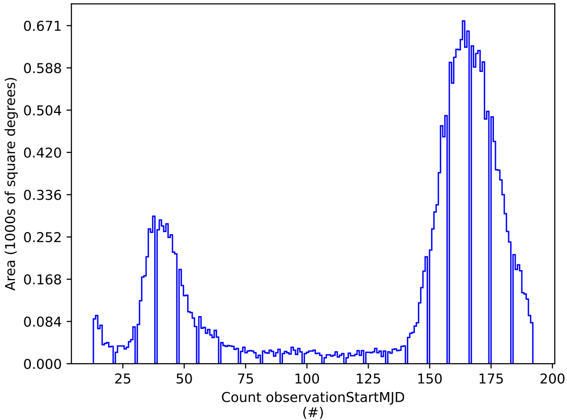
weather_cloudso0v3.5_10yrs z: Count observationStartMJD
