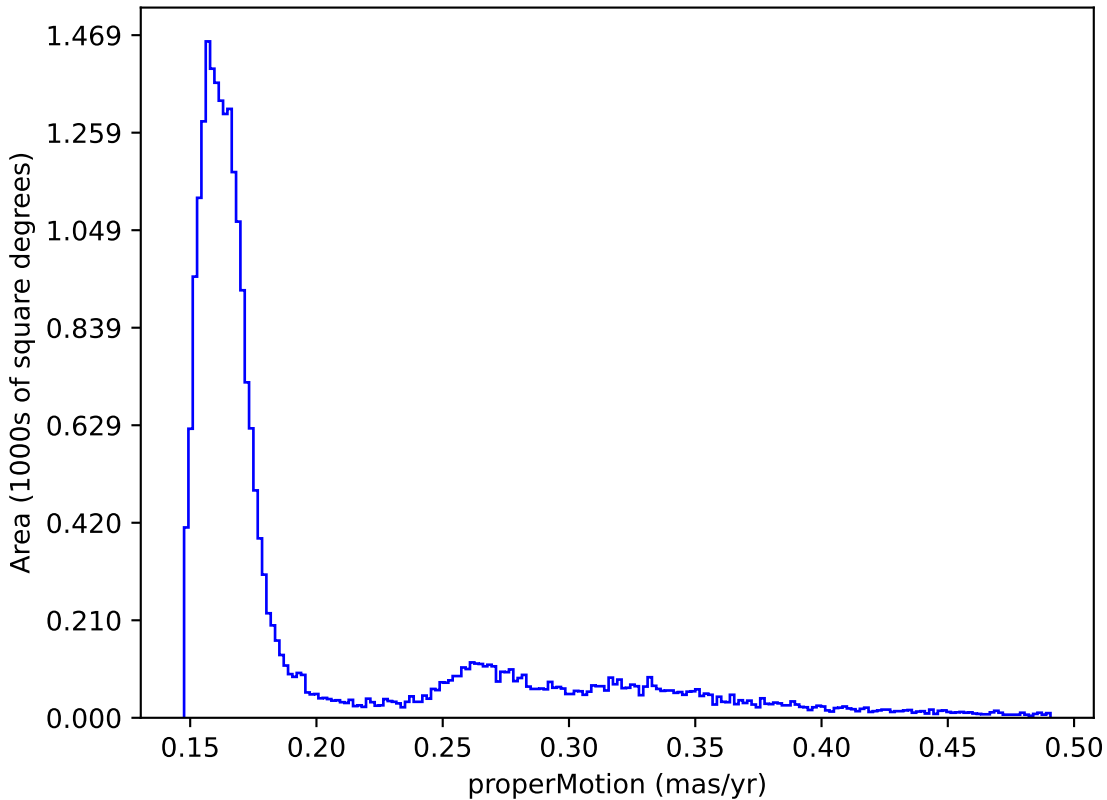
weather_cloudso0v3.5_10yrs : properMotion
