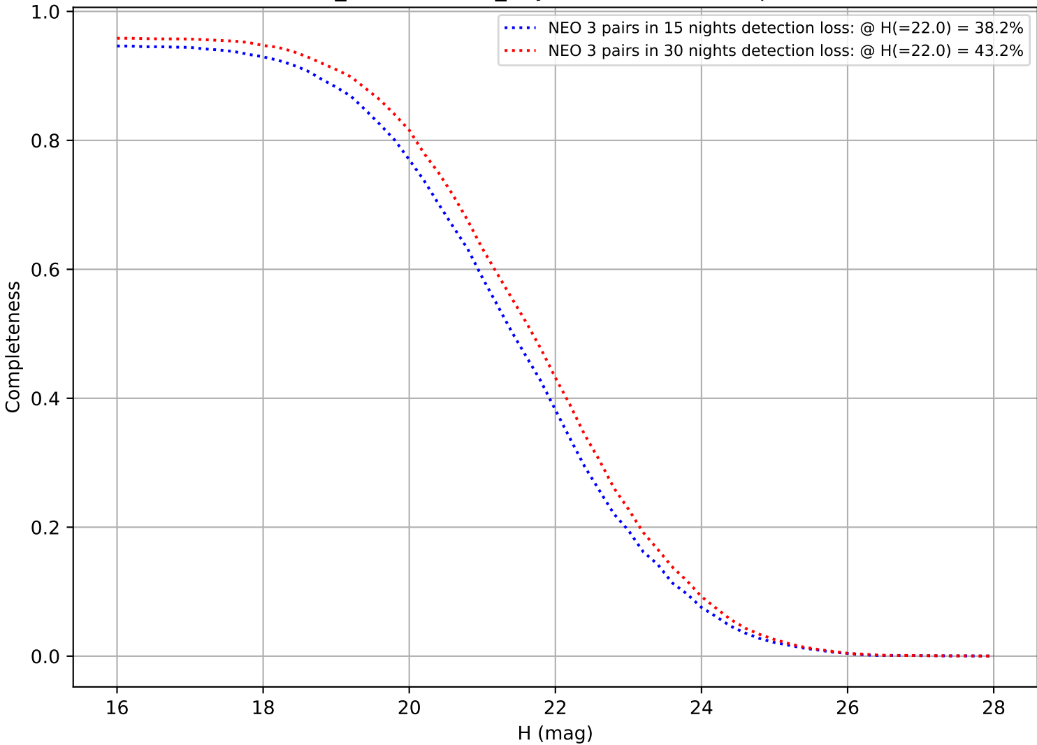
weather_cloudso0v3.5_10yrs: DifferentialCompleteness
