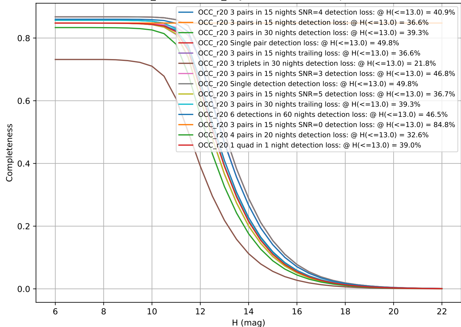
weather_cloudso0v3.5_10yrs: CumulativeCompleteness
