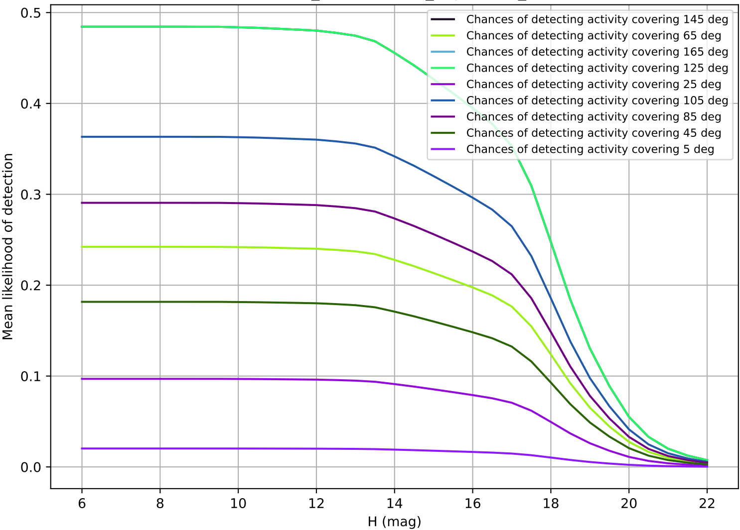
weather_cloudso0v3.5_10yrs OCC_r5
