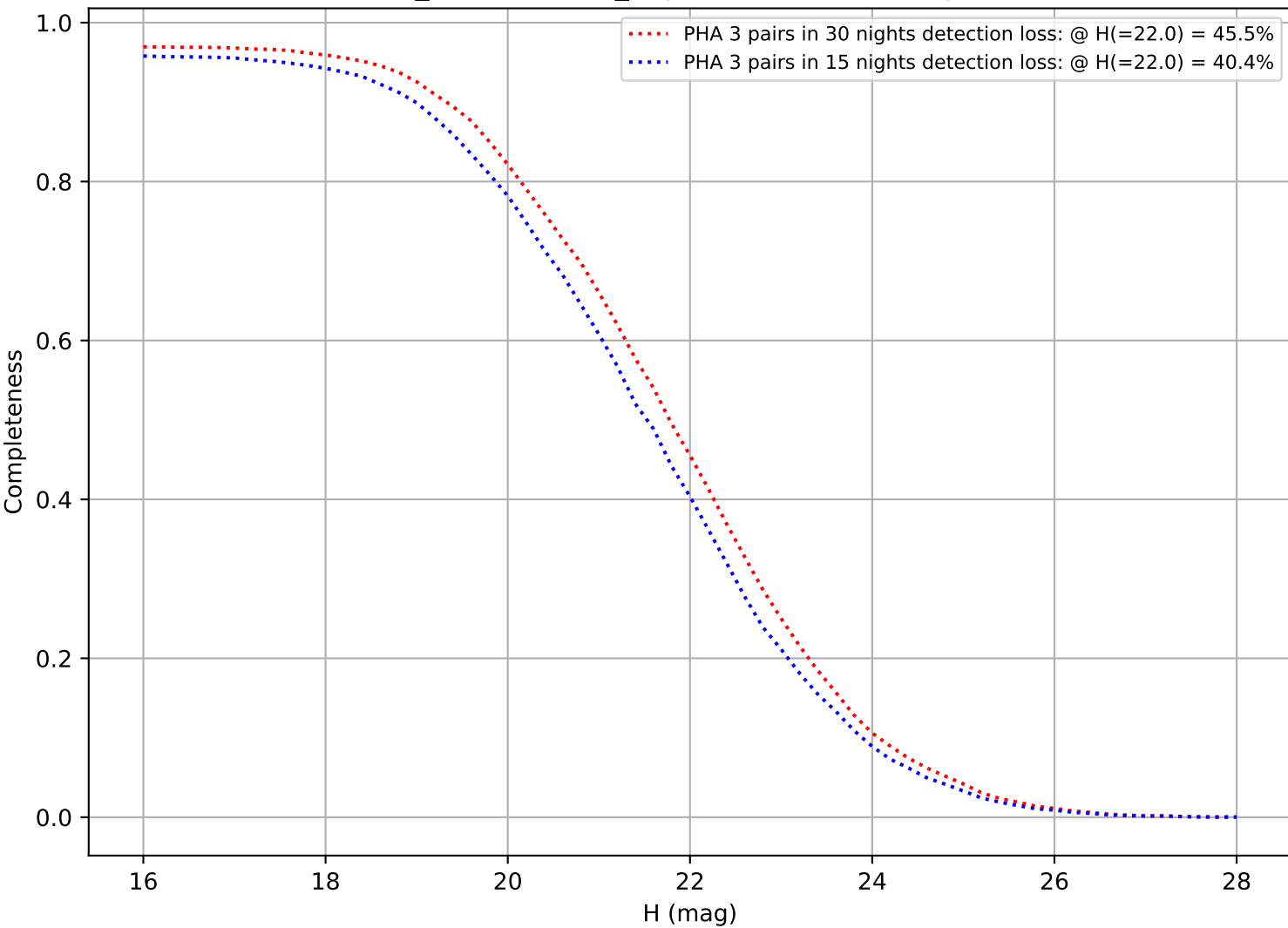
weather_cloudso0v3.5_10yrs: DifferentialCompleteness
