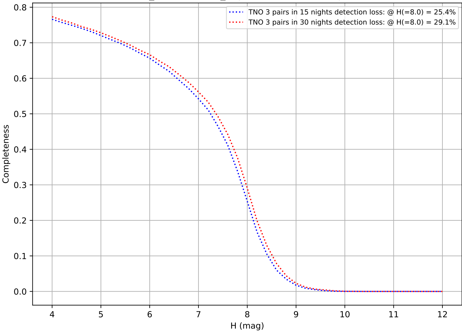
weather_cloudso0v3.5_10yrs: DifferentialCompleteness
