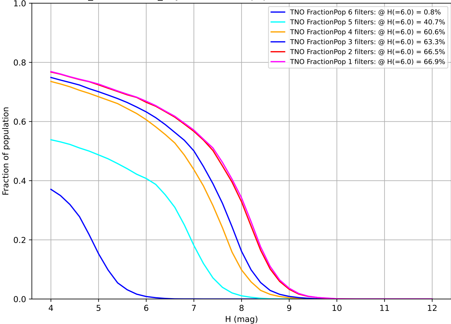
weather_cloudso0v3.5_10yrs: Fraction of population with colors in X filters TNO
