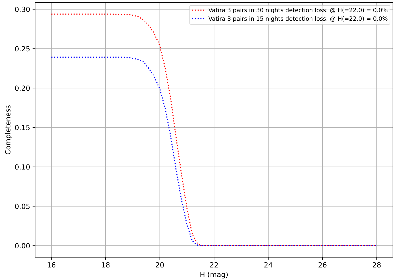
weather_cloudso0v3.5_10yrs: DifferentialCompleteness
