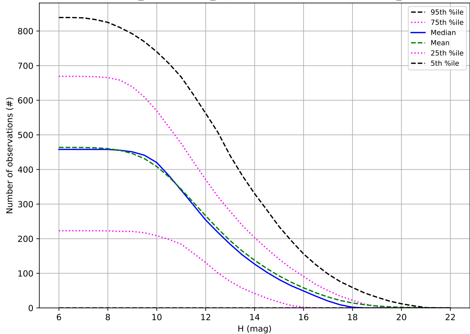
weather_cloudso0v3.5_10yrs: Number of observations OCC_r5
