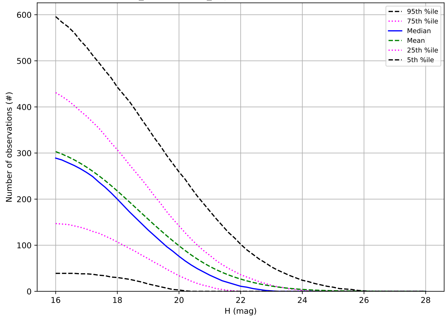
weather_cloudso0v3.5_10yrs: Number of observations PHA
