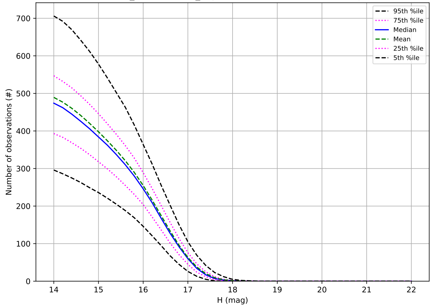
weather_cloudso0v3.5_10yrs: Number of observations Trojan
