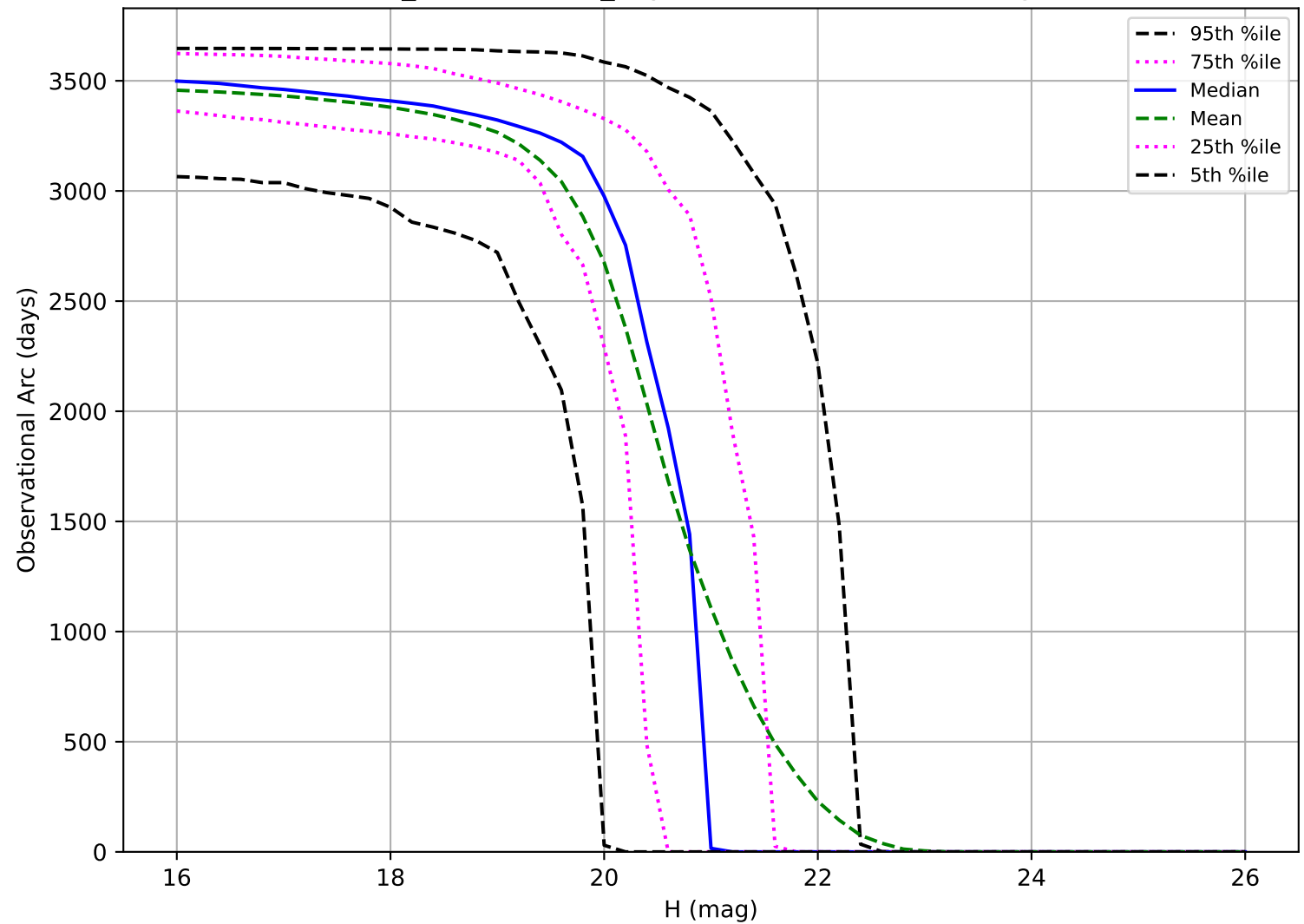
weather_cloudso0v3.5_10yrs: Observational Arc Length MBA
