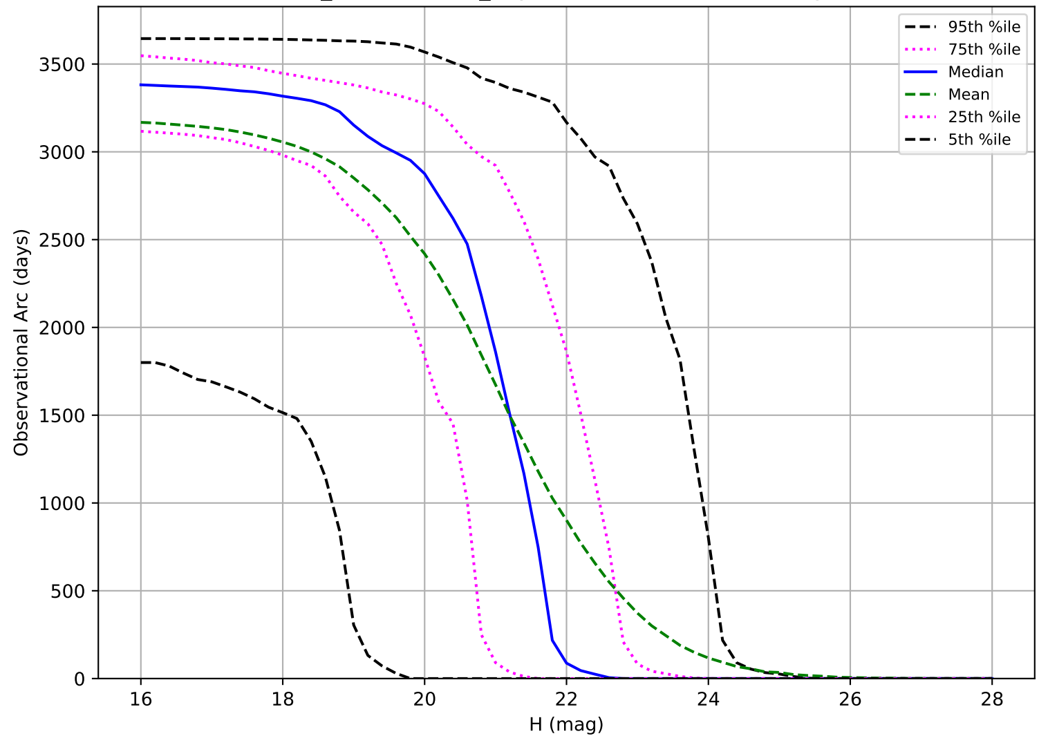
weather_cloudso0v3.5_10yrs: Observational Arc Length NEO
