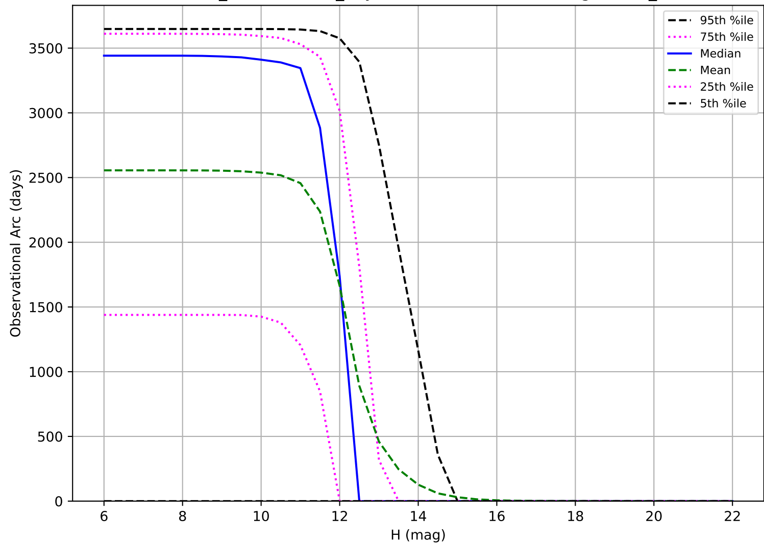
weather_cloudso0v3.5_10yrs: Observational Arc Length OCC_r20
