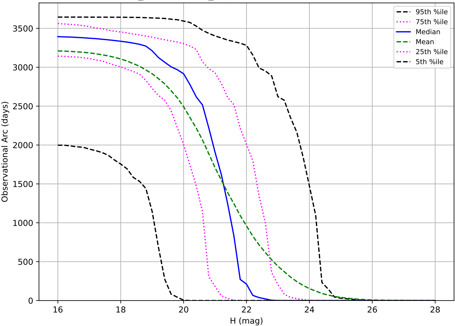
weather_cloudso0v3.5_10yrs: Observational Arc Length PHA
