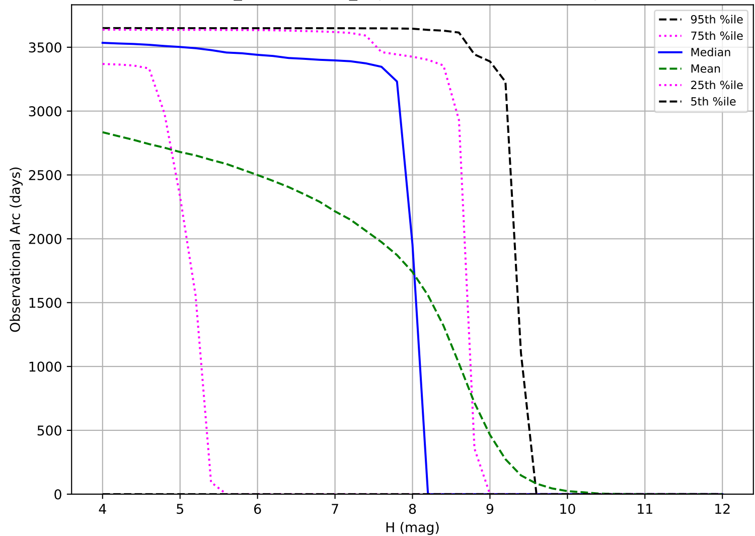
weather_cloudso0v3.5_10yrs: Observational Arc Length TNO
