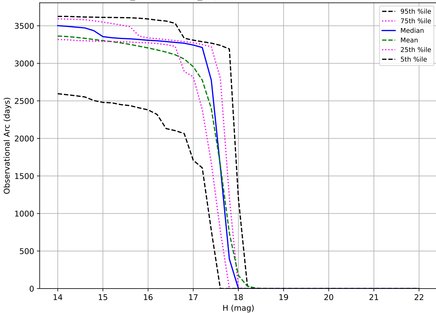
weather_cloudso0v3.5_10yrs: Observational Arc Length Trojan
