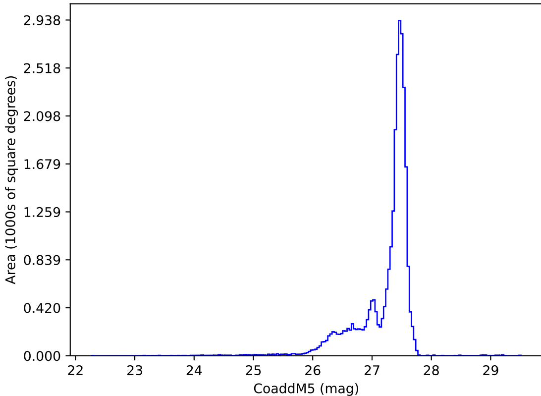
weather_cloudso10v3.5_10yrs : CoaddM5
