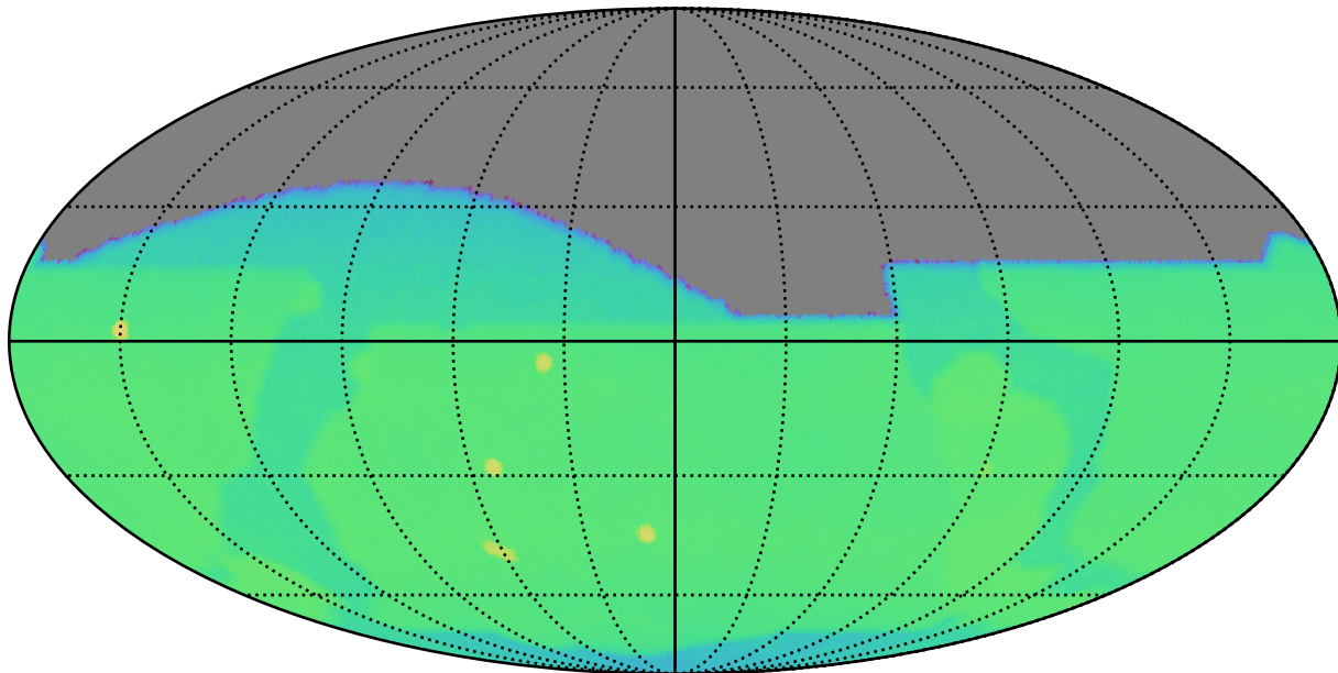
weather_cloudso10v3.5_10yrs : CoaddM5
