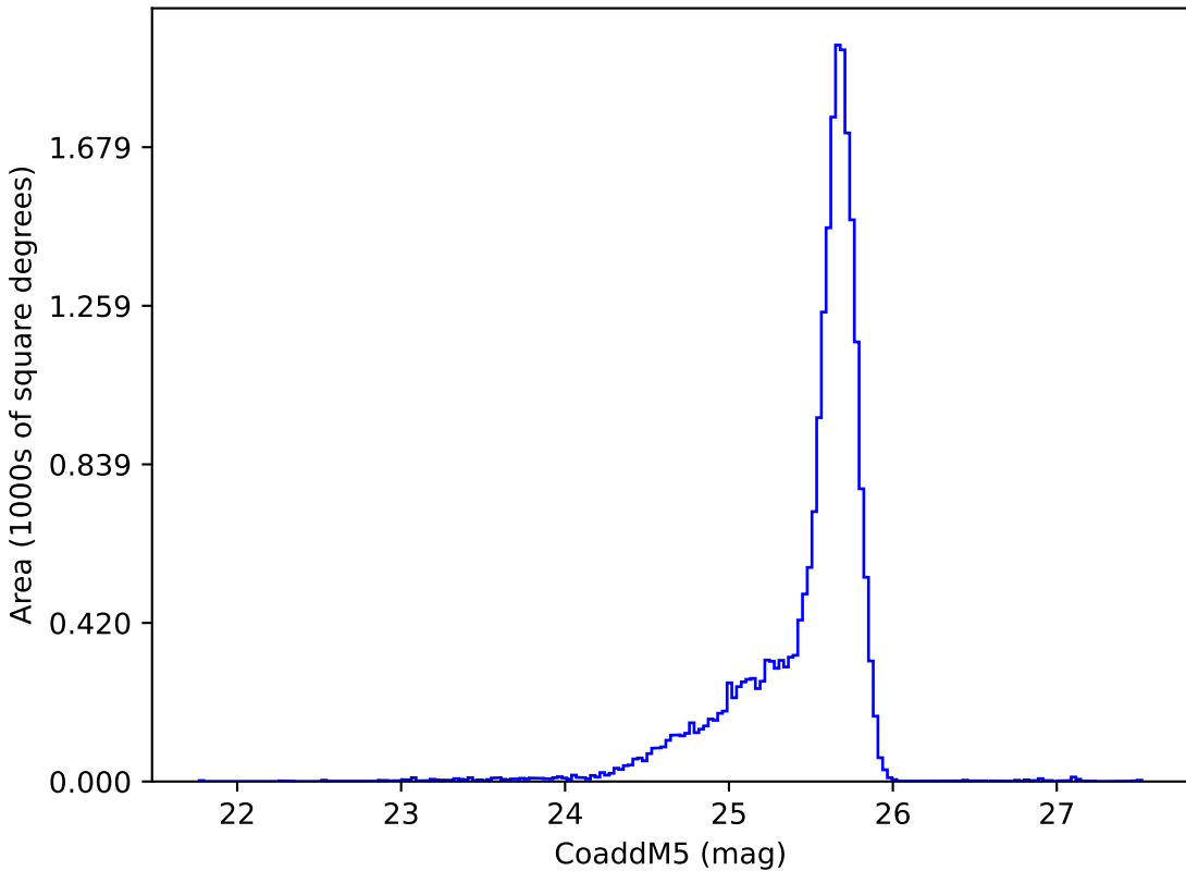
weather_cloudso10v3.5_10yrs u: CoaddM5
