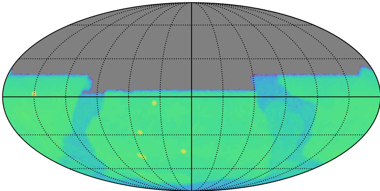
weather_cloudso10v3.5_10yrs u: CoaddM5
