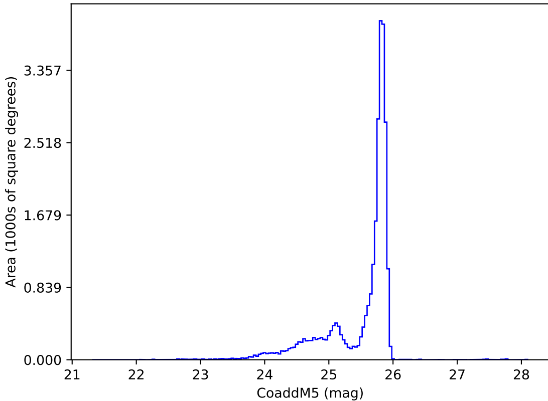
weather_cloudso10v3.5_10yrs z: CoaddM5
