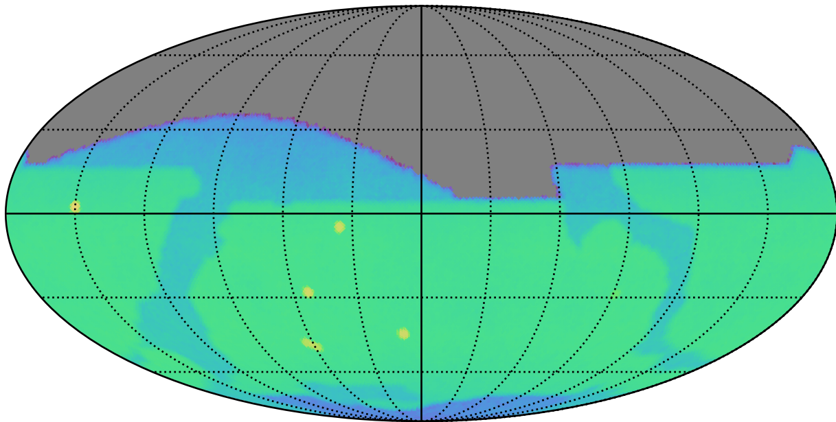
weather_cloudso10v3.5_10yrs z: CoaddM5
