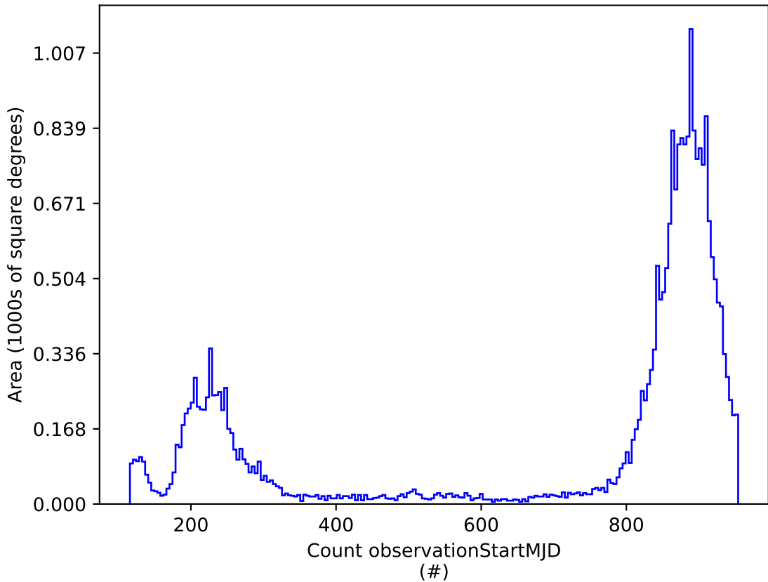
weather_cloudso10v3.5_10yrs : Count observationStartMJD
