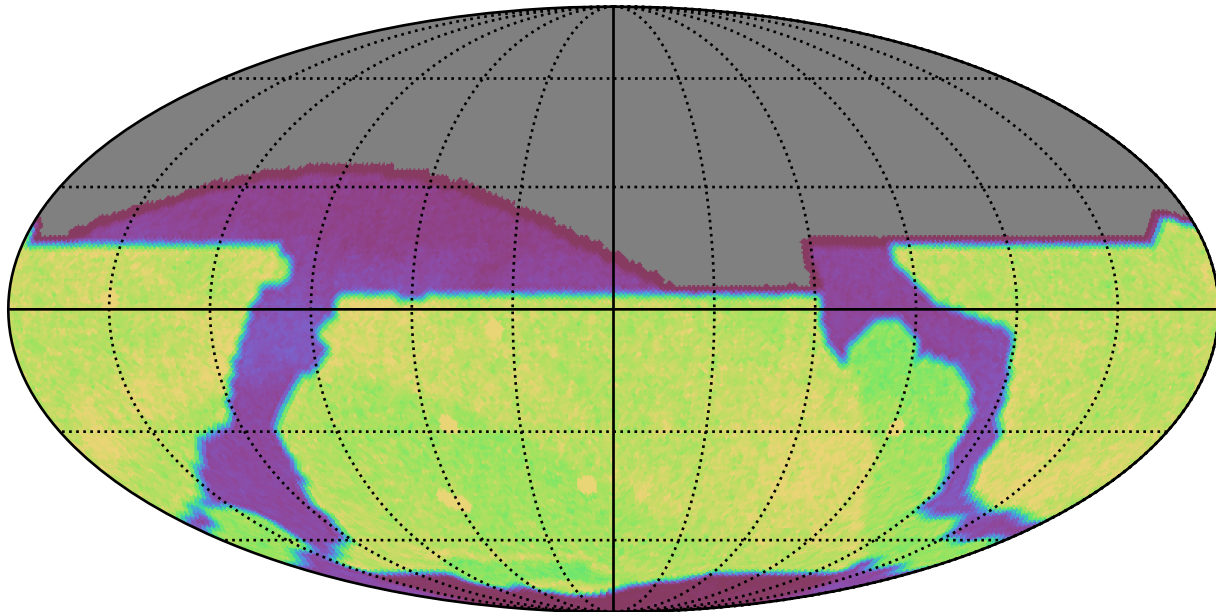
weather_cloudso10v3.5_10yrs : Count observationStartMJD
