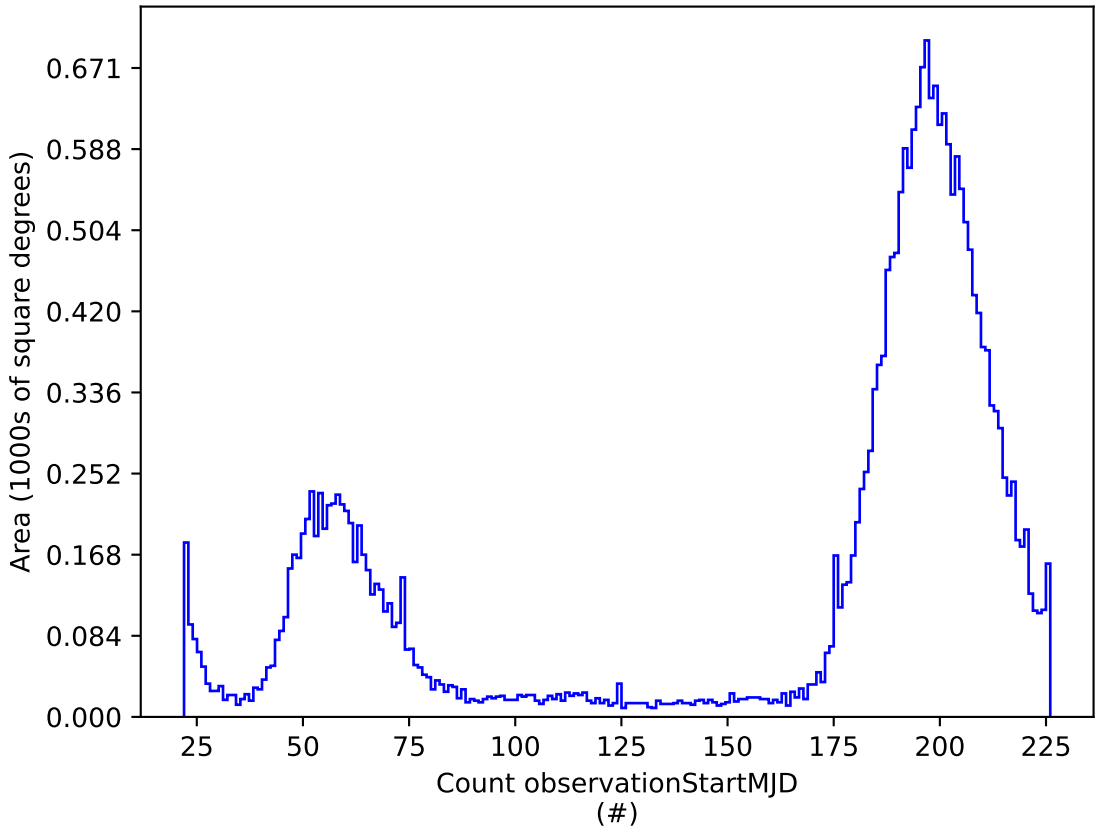
weather_cloudso10v3.5_10yrs i: Count observationStartMJD
