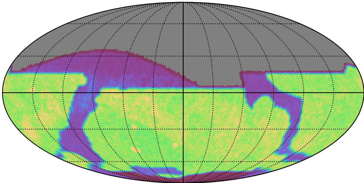
weather_cloudso10v3.5_10yrs z: Count observationStartMJD
