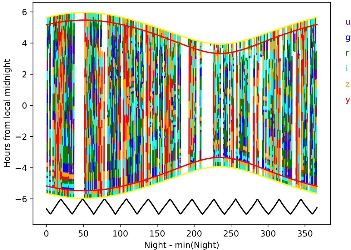
weather_cloudso10v3.5_10yrs year 2-3: Hourglass
