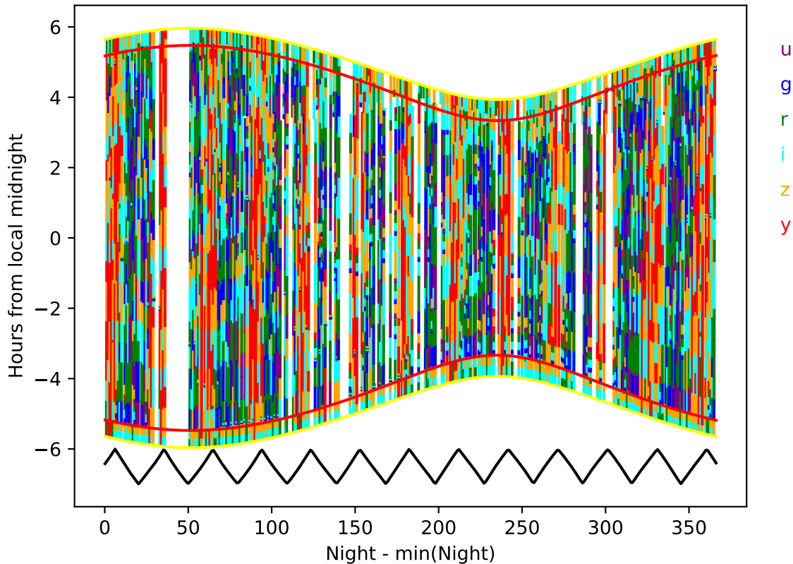
weather_cloudso10v3.5_10yrs year 6-7: Hourglass
